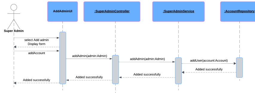
Figure 25: Add Admin Detailed System Sequence
