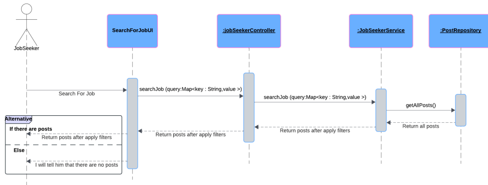
Figure 34: Search For a Job Detailed Sequence Diagram
