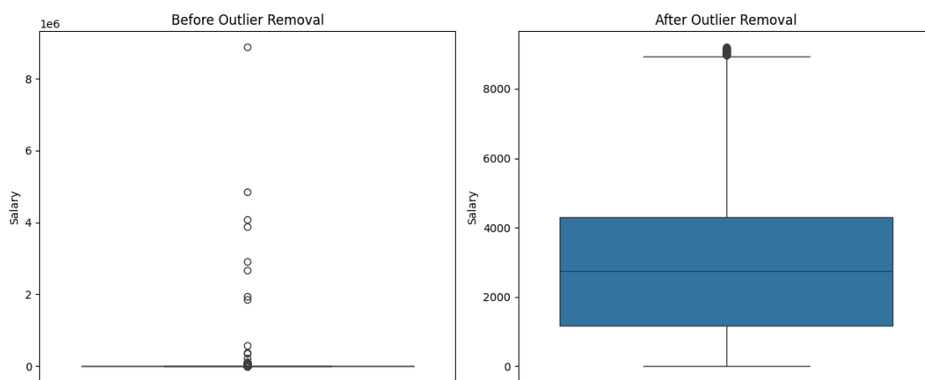
Figure 43: Difference Between Before & After Outlier Removal
