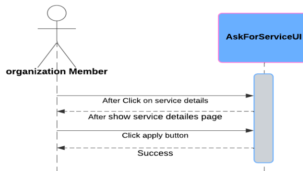
Figure 16: Ask For a Service System Sequence Diagram
