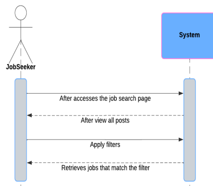
Figure 21: Search For a Job System Sequence Diagram
