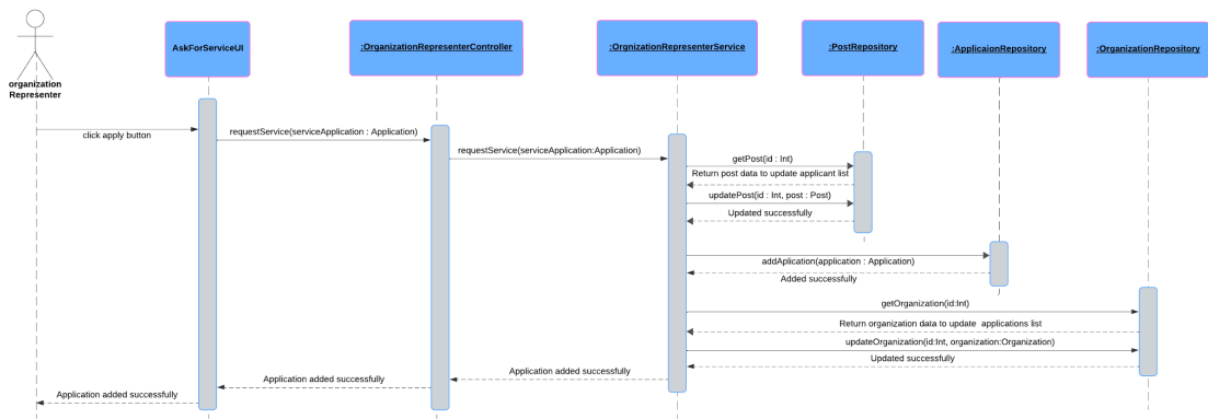
Figure 29: Ask For a Service Detailed Sequence Diagram
