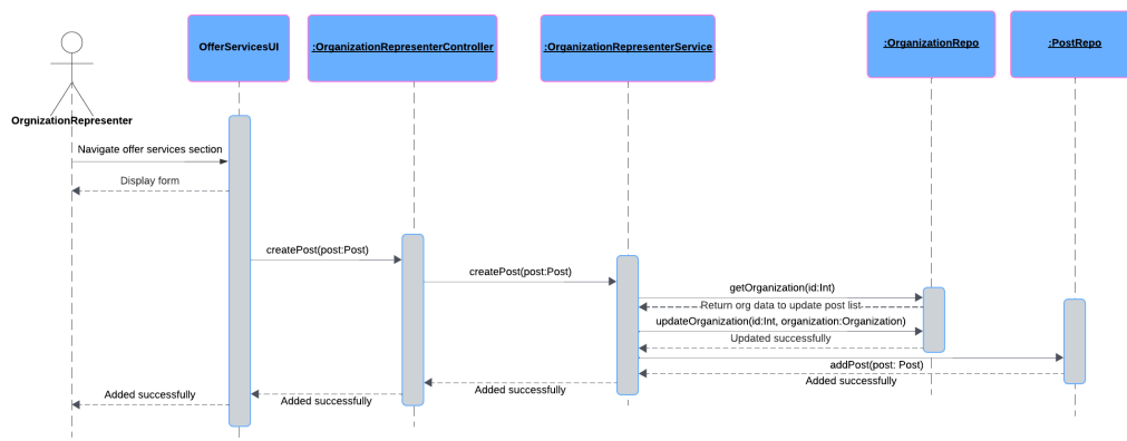
Figure 33: Offer a Service Detailed Sequence Diagram
