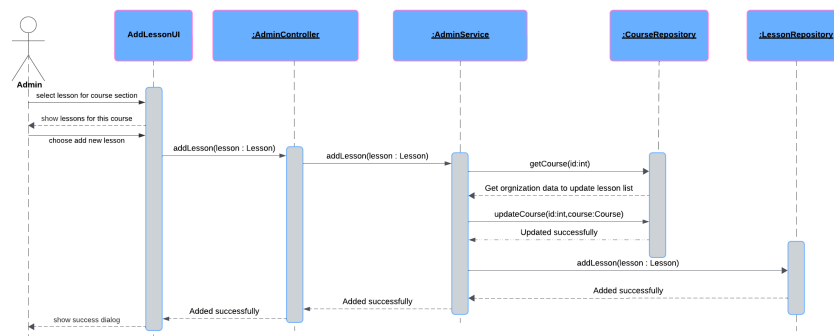
Figure 26: Add lesson Detailed Sequence Diagram
