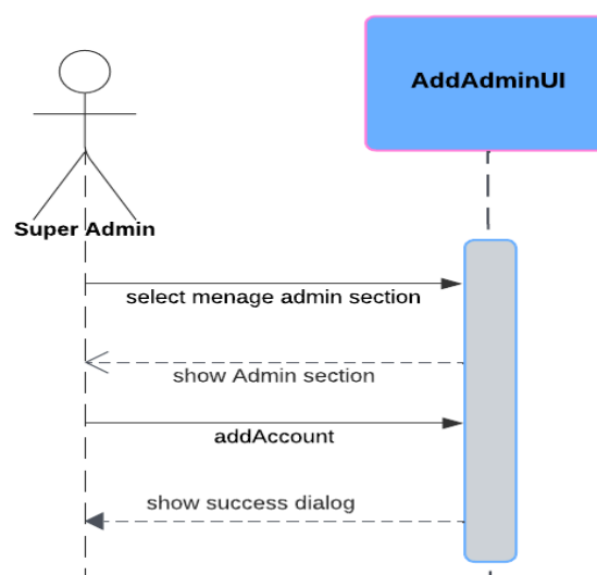
Figure 12: Add Admin System Sequence Diagram
