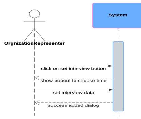
Figure 22: Set Interview Time System Sequence Diagram
