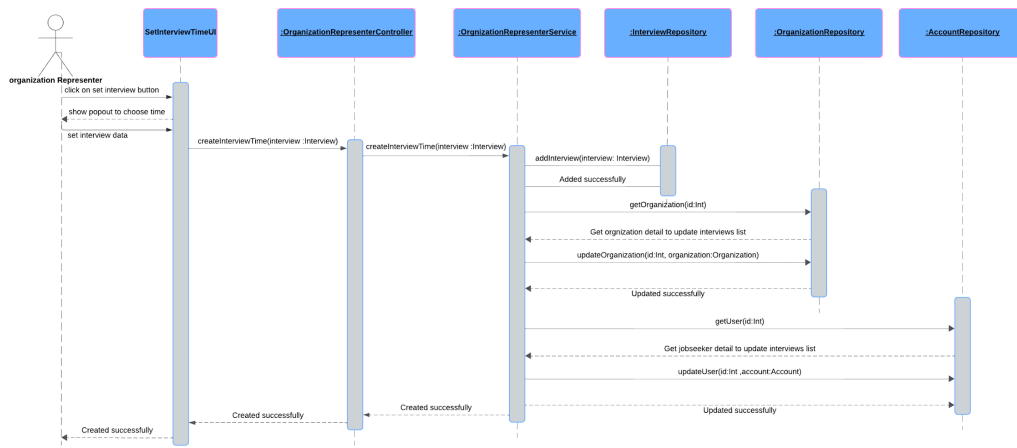
Figure 35: Set Interview Time Detailed Sequence Diagram
