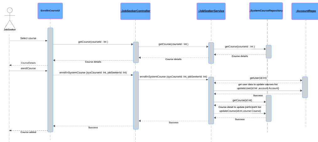
Figure 30: Enroll In a Course Detailed Sequence Diagram
