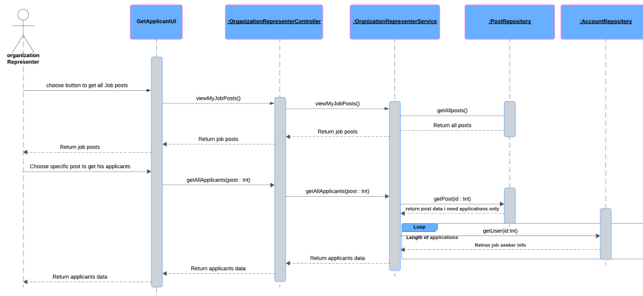
Figure 32: Get Applicants For a Job Detailed Sequence Diagram
