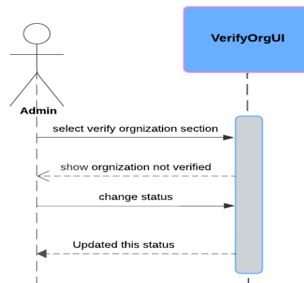
Figure 23: Verify Organization System Sequence Diagram
