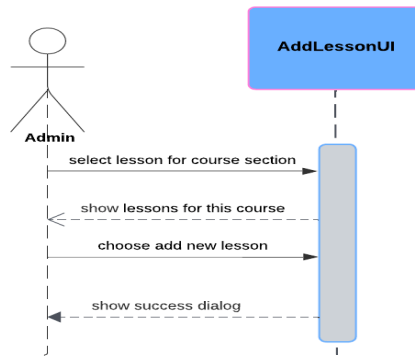
Figure 13: Add lesson System Sequence Diagram
