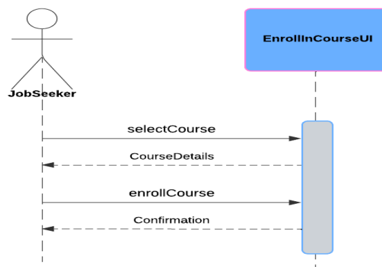
Figure 17: Enroll In a Course System Sequence Diagram
