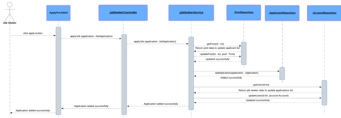
Figure 28: Apply For a Job Detailed Sequence Diagram
