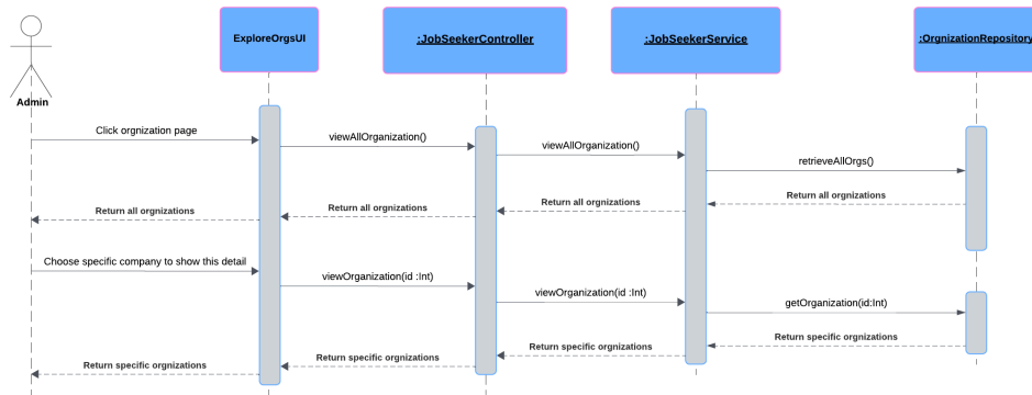
Figure 31: Explore Organizations Detailed Sequence Diagram
