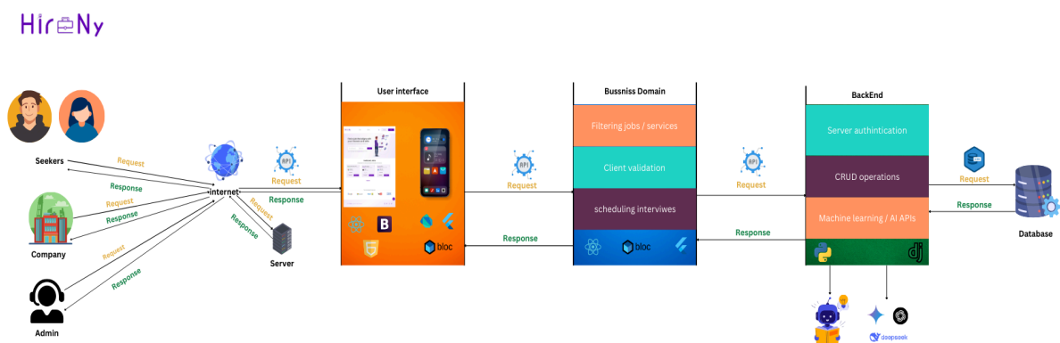
Figure 7: System Architecture Diagram
