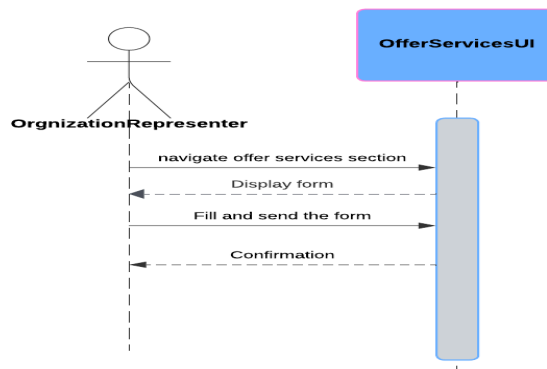
Figure 20: Offer a Service System Sequence Diagram
