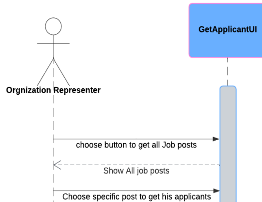
Figure 19: Get Applicants For a Job System Sequence Diagram
