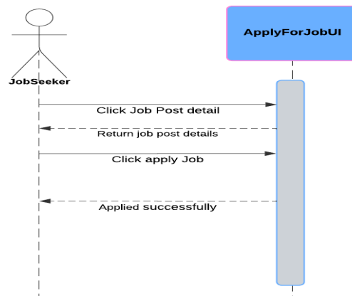
Figure 15: Apply For a Job System Sequence Diagram
