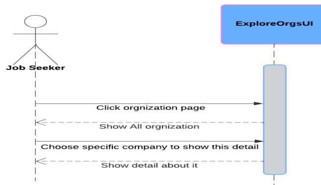
Figure 18: Explore Organizations System Sequence Diagram
