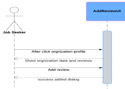
Figure 14: Add Review System Sequence Diagram
