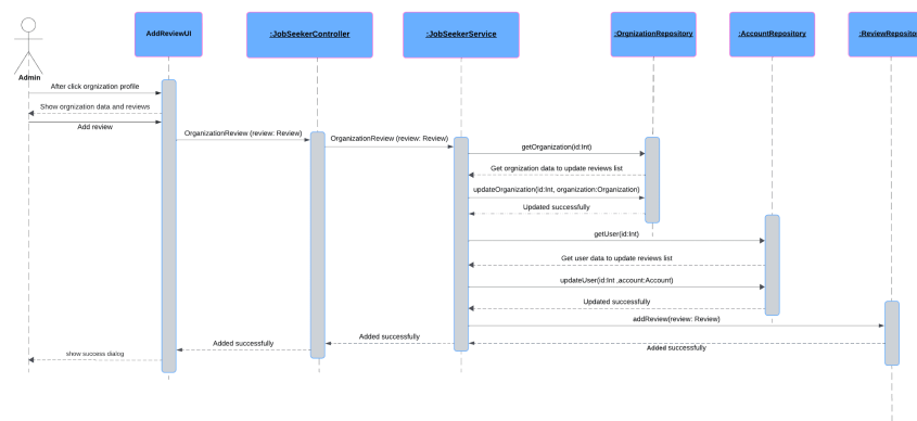
Figure 27: Add Review Detailed Sequence Diagram
