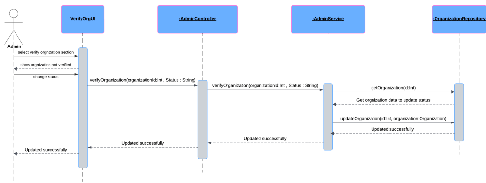
Figure 36: Verify Organization Detailed Sequence Diagram
