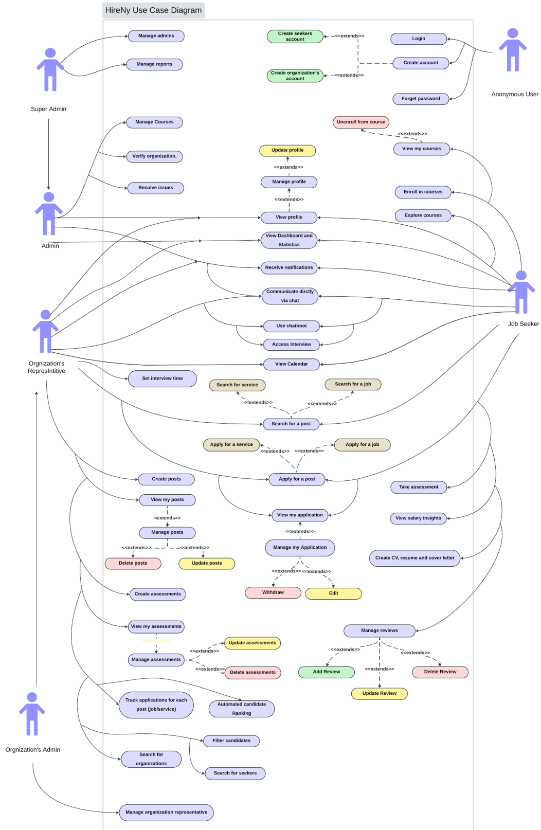
Figure 8: Use Case Diagram
