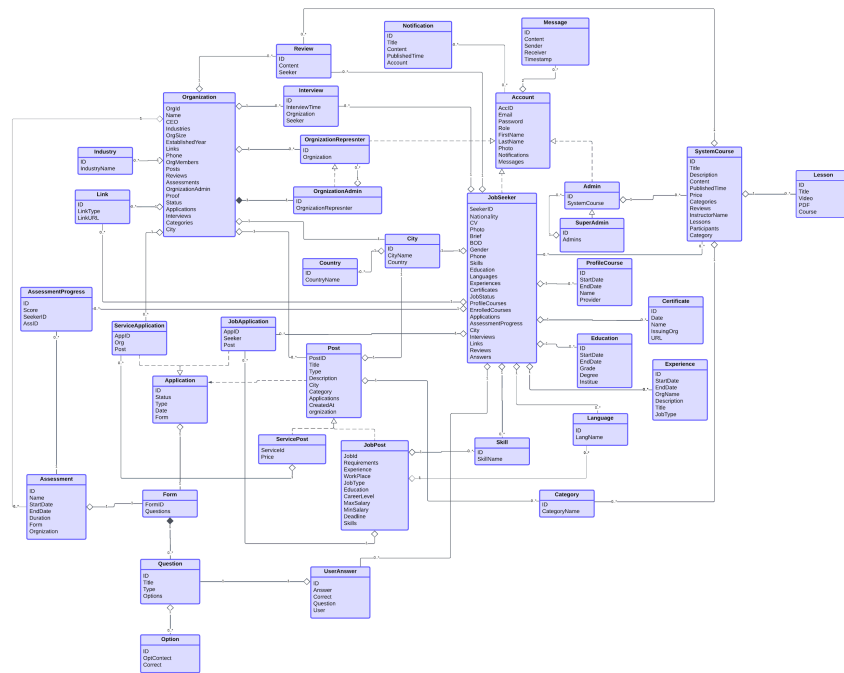
Figure 9: Domain Class Diagram
